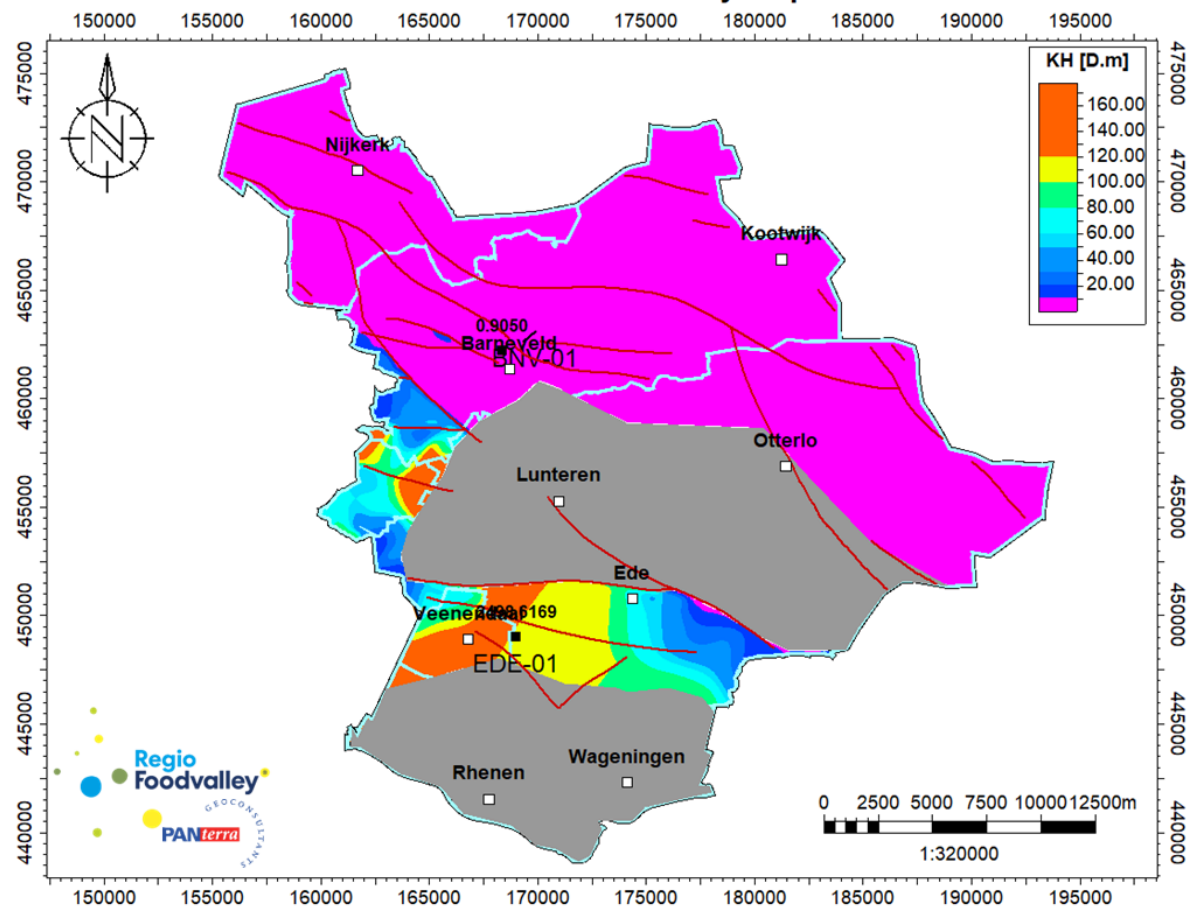
Slochteren Transmissivity Map
