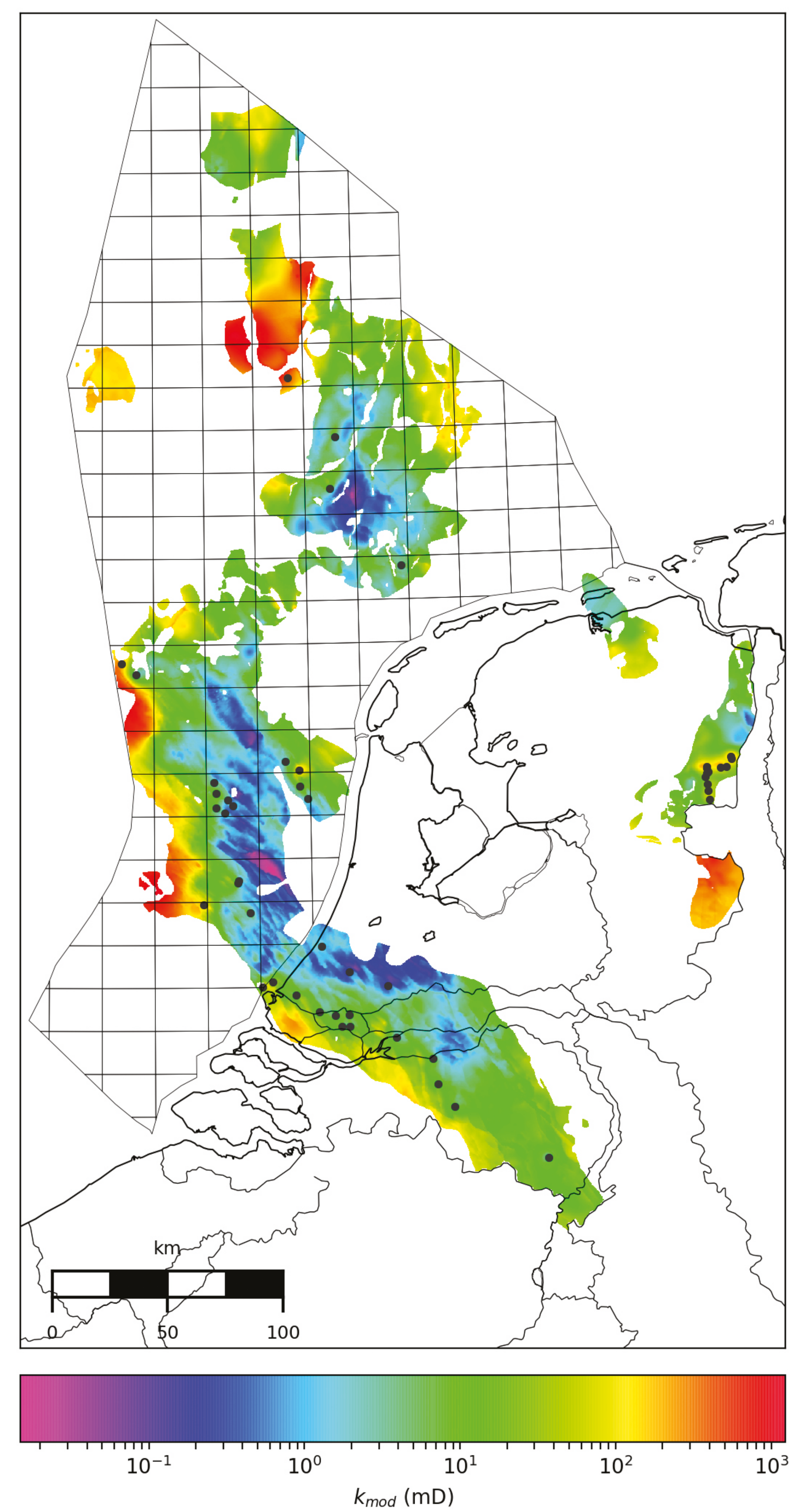
Figure 2. Permeability map of the Triassic Lower Detfurth Sandstone formation (RBMDL).
