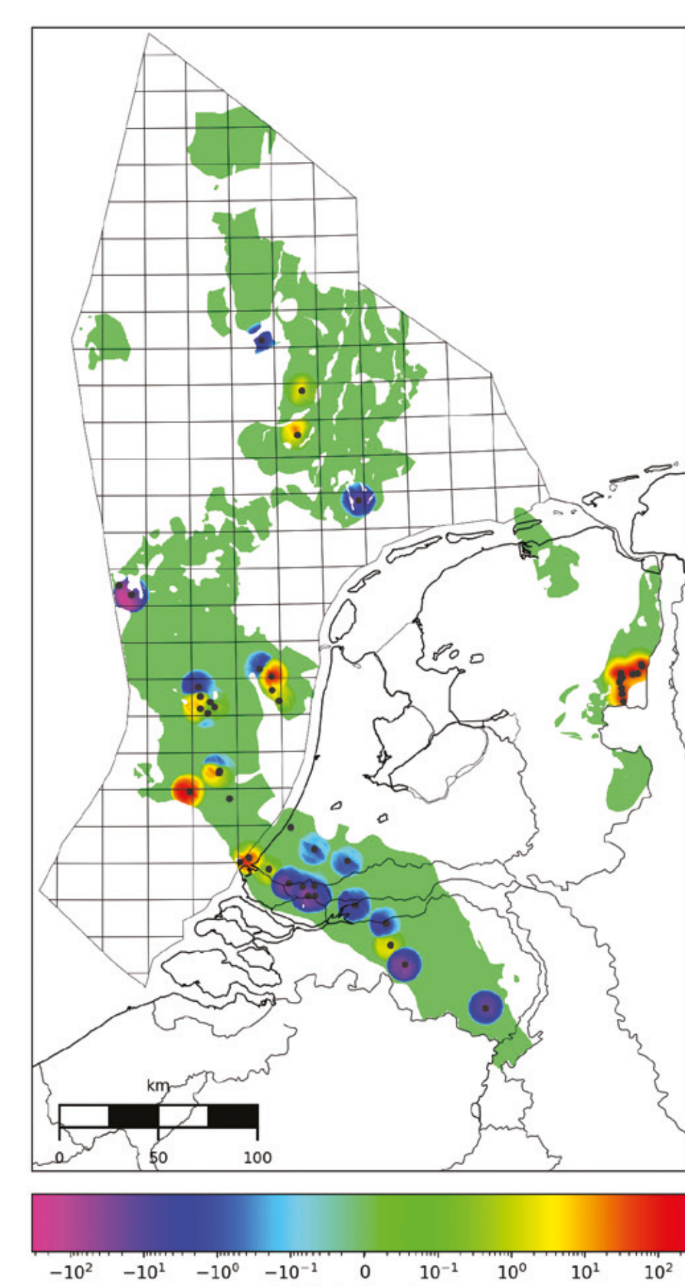
Figure 6. Residual permeability map for the Lower Detfurth Sandstone formation.
