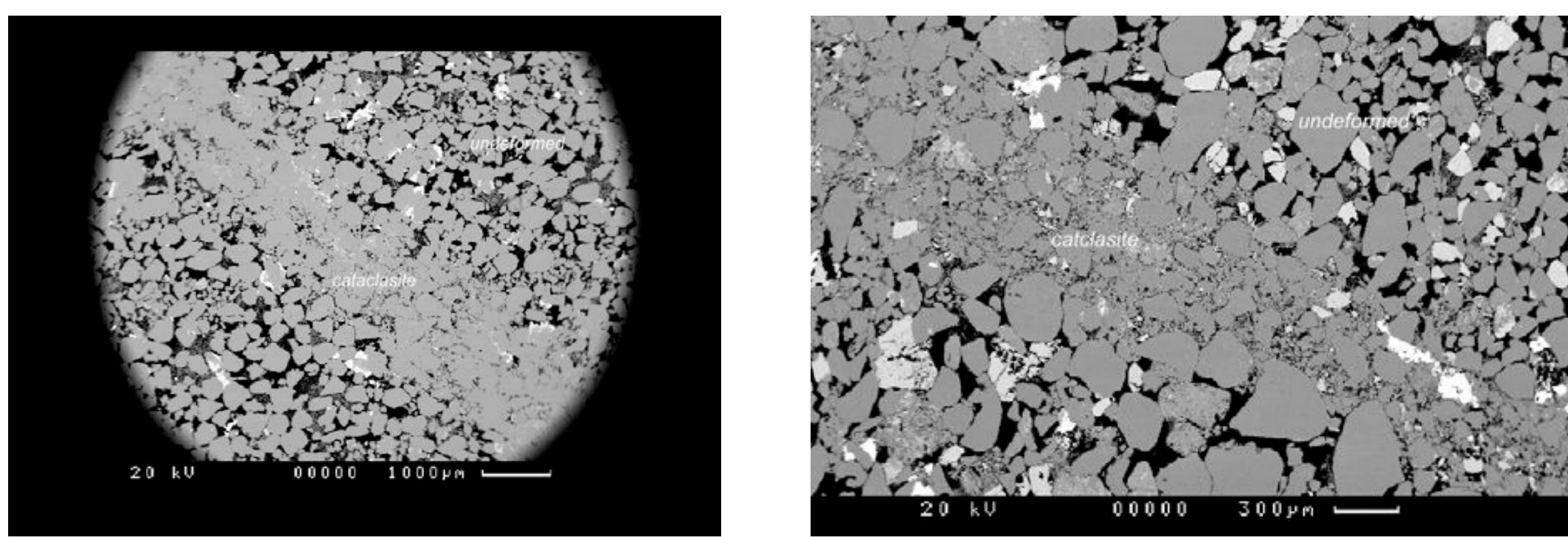
Figure 3. Very low magnification BSE micrographs of a cataclastic fault rock and its host sandstone. (Zeilstra et al., 2007)
